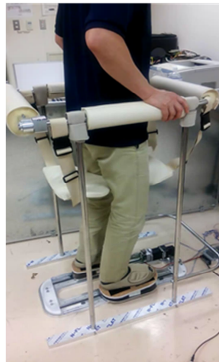
Fig. 3 The training robot for the basic walking pattern for home use. The robot has simplified functions and mechanisms, and a robust and easy to use user interface. The light weight, low cost and safety are important for the home use
