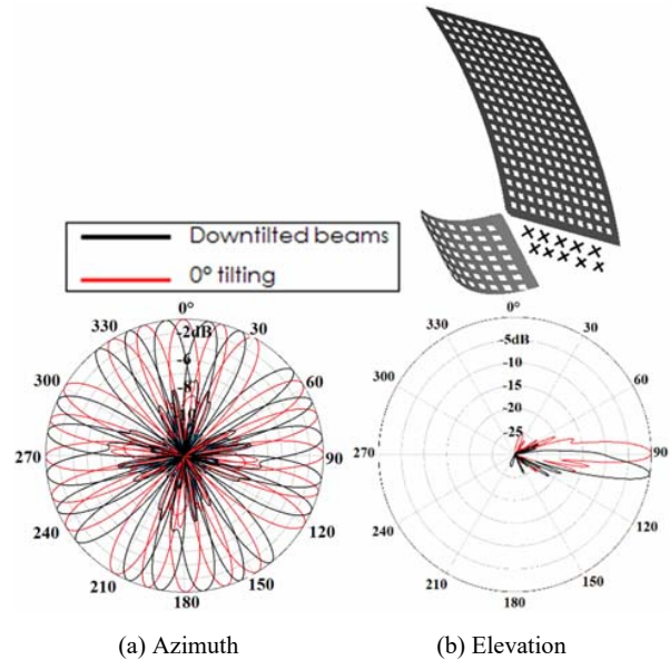
Fig. 8 Four penta beam units covering 360^\circ with 40 beams at a sample frequency 4 GHz
