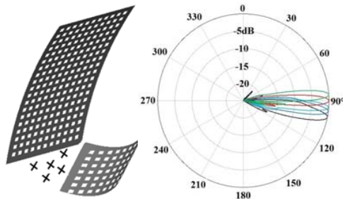
(a) Five feeds with different elevations (b) Elevation patterns Fig. 3 A penta beam antenna generating five beams with different elevation angles
