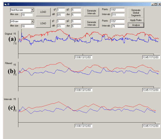
Fig. 4 ABSTRACTOR applied to environmental data
