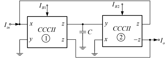
Fig. 3 Proposed current-mode first-order allpass filter
