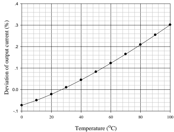
Fig. 9 The amplitude deviation of the output current for temperature variations
