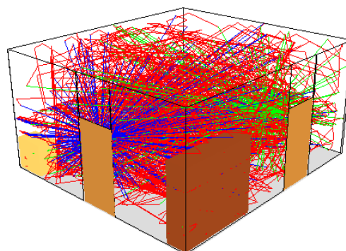
Fig. 3 Visible rays received by receiver inside room
