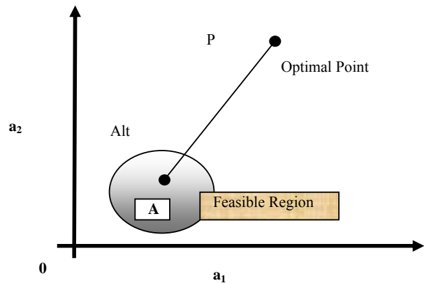
Fig. 1 Distance based approach
