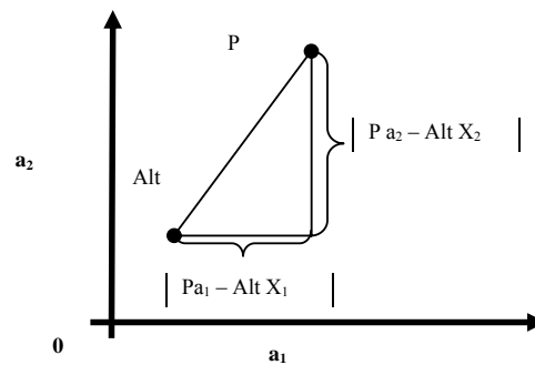
Fig. 2 Distance of real vector
