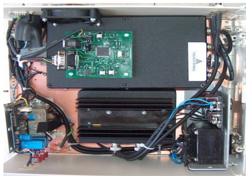
Fig. 6 RFID Radar (reader) circuit board
