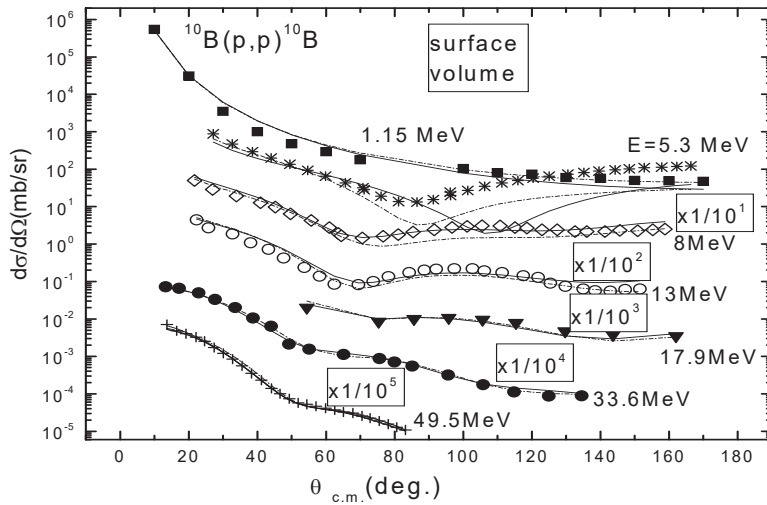
Fig. 1 Angular distribution for protons elastically scattered by 10 B at different energies. The solid curves are calculations based on volume absorption W_v (set A of Table I); dashed calculations are based on surface absorption W_s (set B of Table I); experimental data are the points which were taken from [17]-[20]
