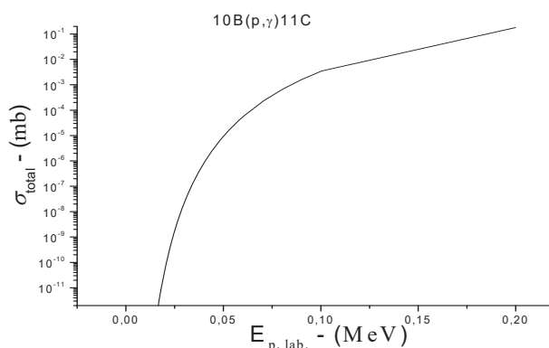
Fig. 4 Calculated cross sections of {}^{10}\text{B}(p,\gamma){}^{11}\text{C} reaction
