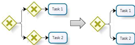
Fig. 4 Refactoring Operator 2
