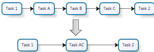
Fig. 11 Refactoring Operator 9
