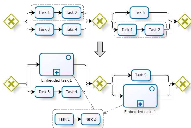
Fig. 6 Refactoring Operator 4
