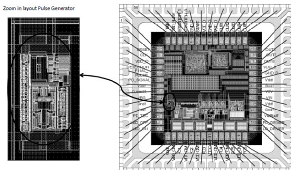
Fig. 11 Layout Drawing of the Tapeout Pulse Generator
