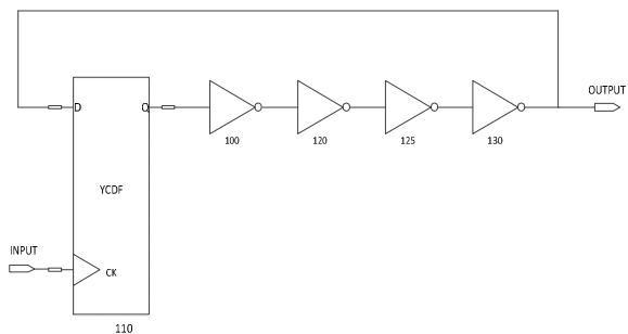
Fig. 5 Frequency Divider Schematic Diagram
