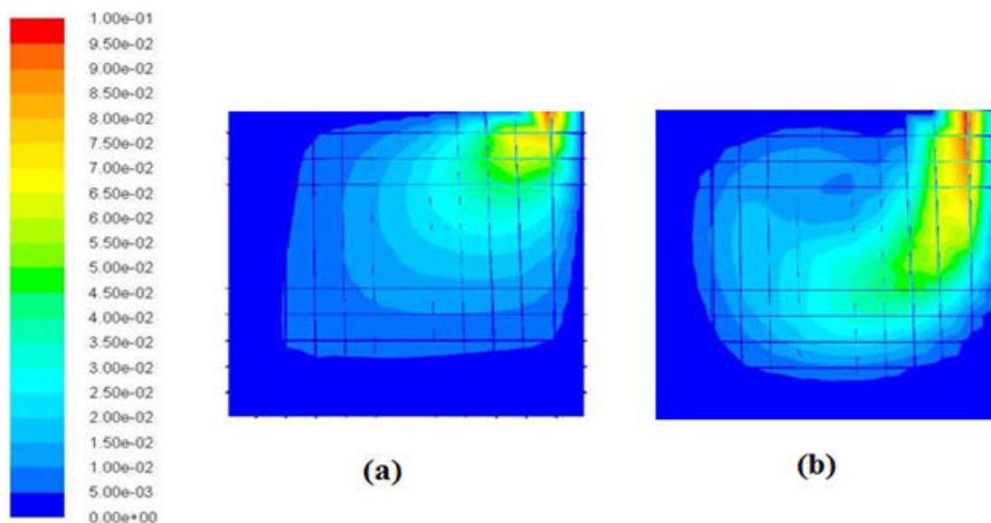
Fig. 11 Velocity contour at different heat transfer coefficient for t = 10 \text{ sec} , v_i = 0.1 \text{ m/s} , T_i = 973 \text{ K} , T_{wl} = 773 \text{ K} , h_g = 5 \text{ cm} and filling at the right side of the top plane: (a) insulated wall and (b) h=20 \text{ w/m}^2\text{K}
