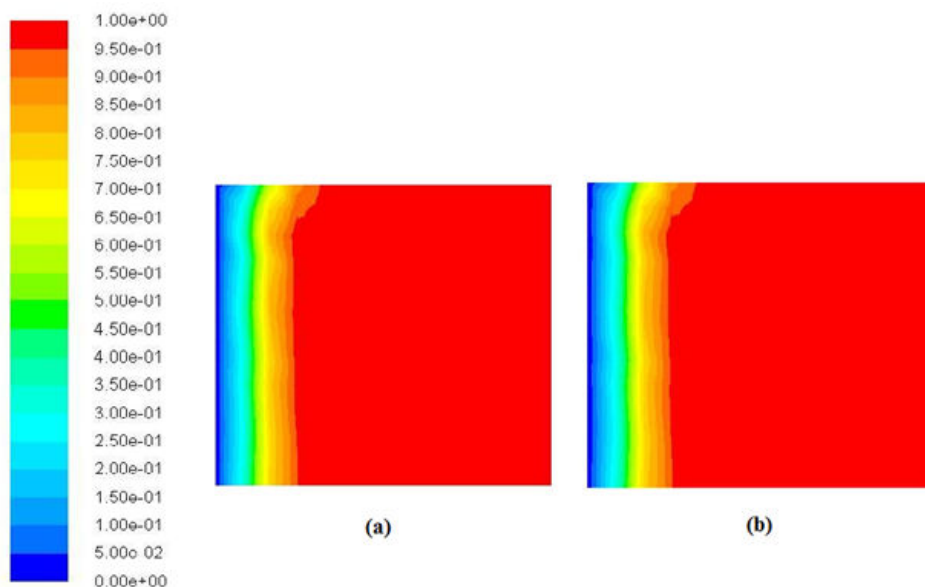
Fig. 12 Liquid fraction contour at different heat transfer coefficient for t = 10 \text{ sec} , v_i = 0.1 \text{ m/s} , T_i = 973 \text{ K} , T_{wl} = 773 \text{ K} , h_g = 5 \text{ cm} and filling at the right side of the top plane (a) insulated wall and (b) h=20 \text{ w/m}^2\text{K}
