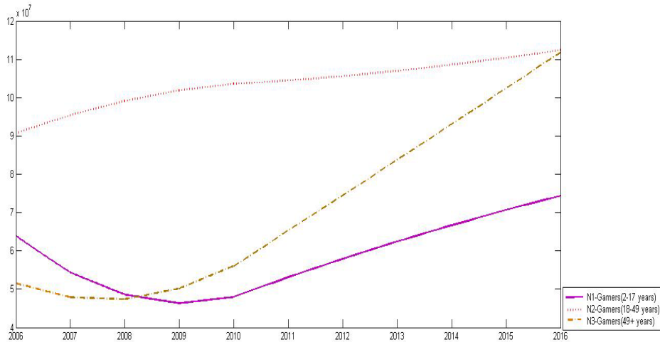
Fig. 3 Model Forecast 2006-2016
