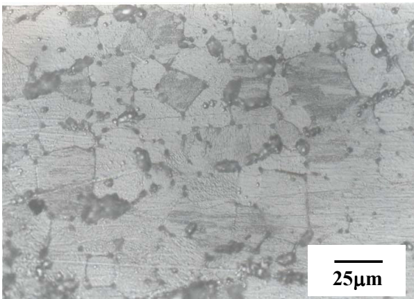
Fig. 13 Optical micrograph of 75% cold rolled alloy 1, aged at 400°C for 1 hour
