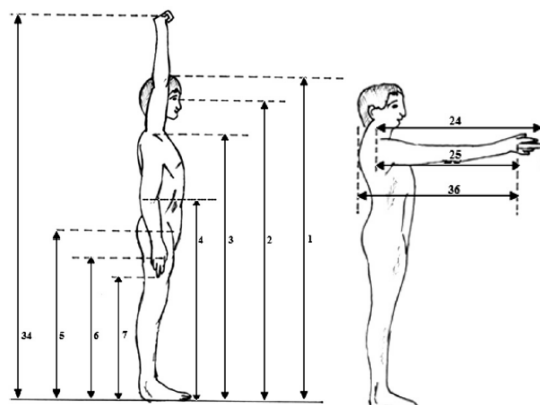
Fig. 1 Size posture with anthropometric Indonesian people in assembly lines
