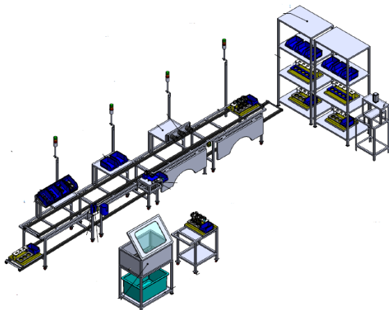
Fig. 10 New piston workstation layout
