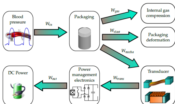
Fig. 9 Energy Flow in Blood Pressure Energy Harvesting
