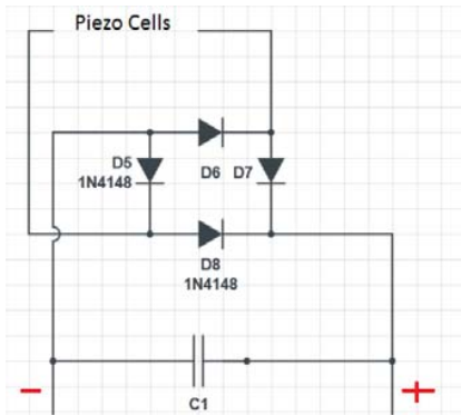
Fig. 7 AC → DC Converter Device
