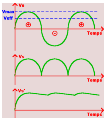
Fig. 8 AC → Obtained Voltage Curves
