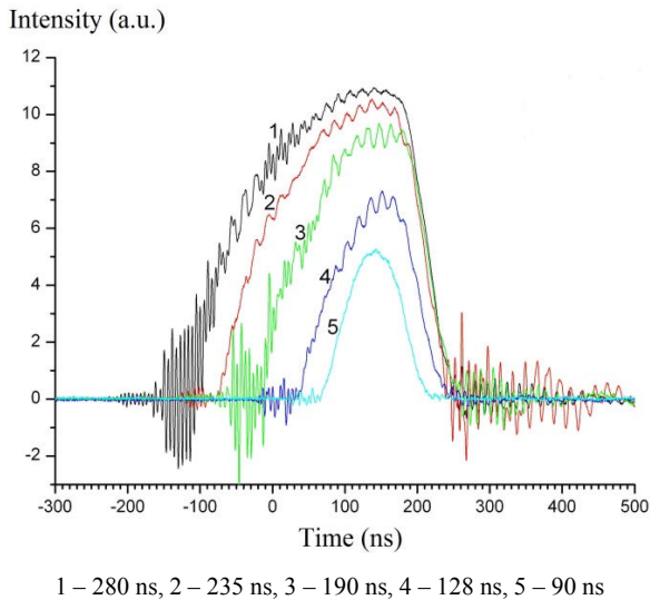
Fig. 2 The LDM radiation pulse amplitude dependence on the pulse duration
