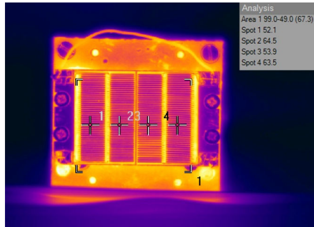
In the right corner of the figure the temperature of individual laser diode array and the LDM mount is presented in Celcius degrees
