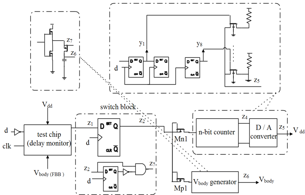
Fig. 2 Expanded proposed V_{DD}/V_{TH} monitoring circuit
