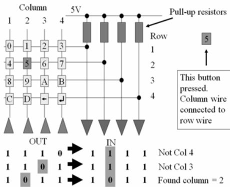
Fig. 1 Keyboard Matrix
