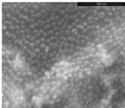
Fig. 3 SEM image of the gold nanoparticles suspension
