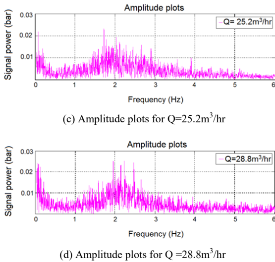
Fig. 4 Plots of pressure fluctuation FFT of the instantaneous pressure
