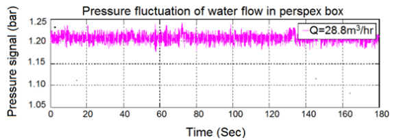
(b) Plot of pressure fluctuation in Perspex box for Q=28.8 m 3 /hr
