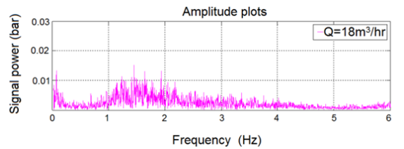
(c) Amplitude plots for Q=18 m 3 /hr
