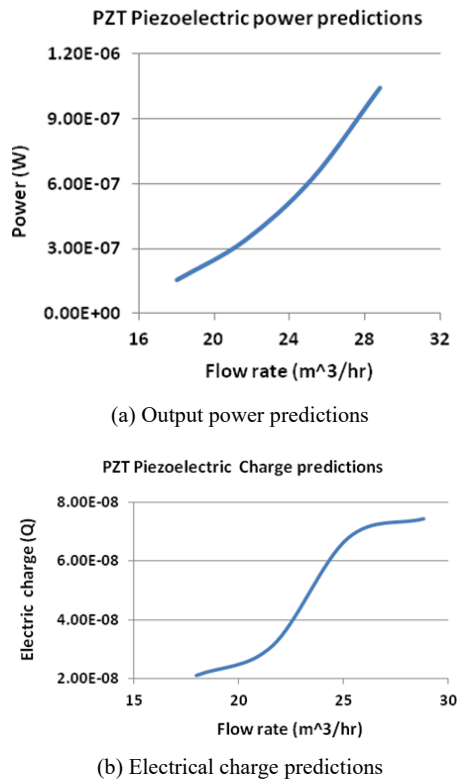
Fig. 6 Predictions of electrical output from PZT Piezoelectric material using single-phase flow
