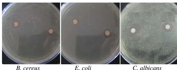
Fig. 5 Inhibition zones of methanolic extract from Salvia officinalis for bacterial strains tested
