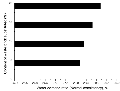
Fig. 2 Variation of the normal consistency cement paste as a function of the content of waste brick
