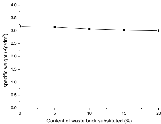
Fig. 1 Variation of the specific weight of cement as a function of the content of waste brick
