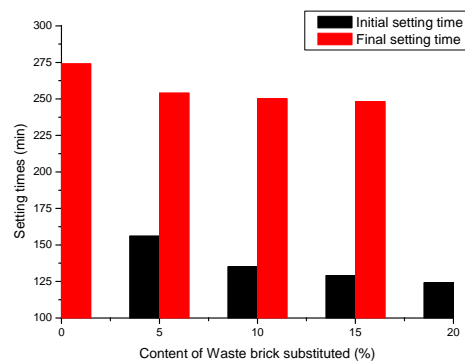
Fig. 3 Variation of the setting times as a function of the content of waste brick
