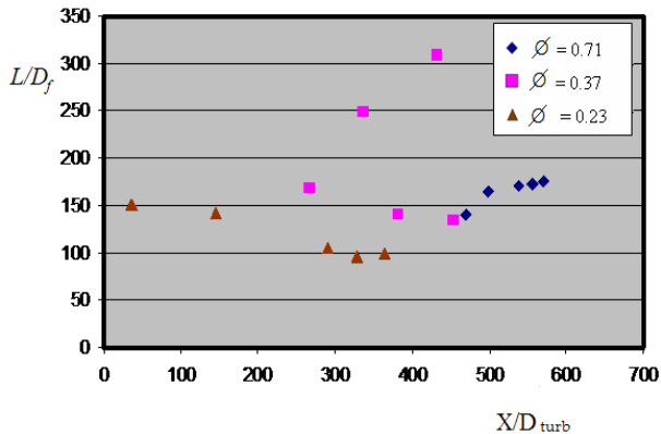
Fig. 9 Dimensionless flame height to extinguishment distance
