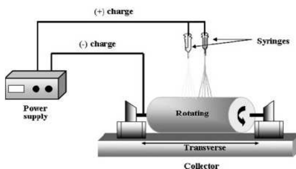
Fig. 1 Schematic diagram of the double-spinneret electrospinning
