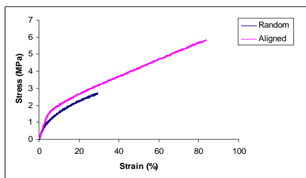
Fig. 3 stress–strain curves for electrospun nanocomposite scaffolds
