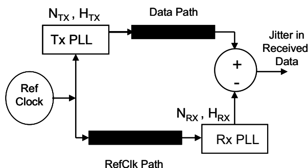
Fig. 1 Generic model of jitter propagation commonly found in high speed data link architecture.
