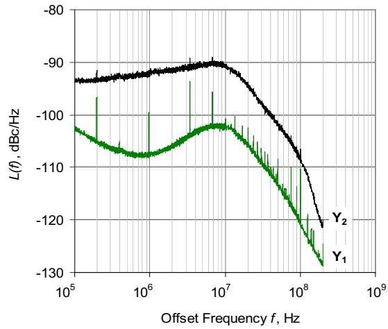
Fig. 6 PLL outputs at 6.4 GHz for the two levels of jitters carried by the input clock.
