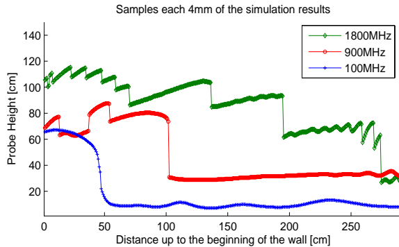
Fig. 4: Threshold over which the influence of the wall on plane wave propagation at 100, 900 and 1800MHz with Horizontal Polarization is under 5% with regard to EM field strength in free space.
