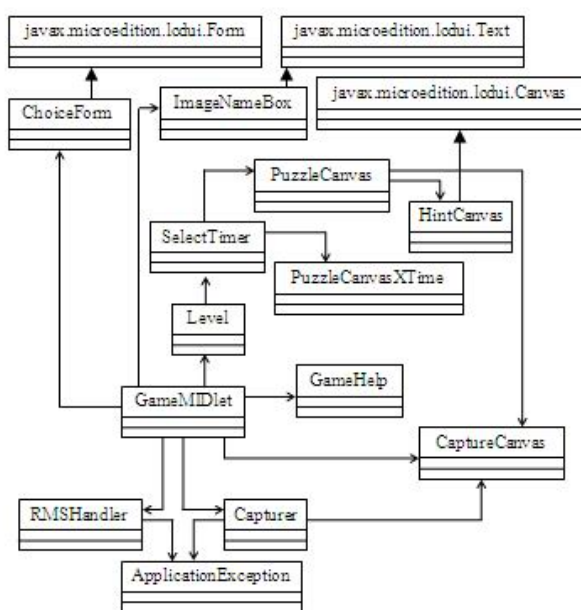
Fig. 2 Class Diagram
