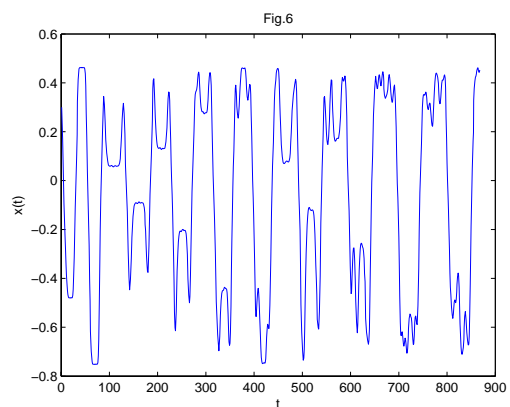
Figs.5-6 Dynamic behavior of system (11): times series of x . A Matlab simulation of chaotic phenomena appears to system (11) with \tau = 12 and \tau = 24 . The initial value is 0.3.
