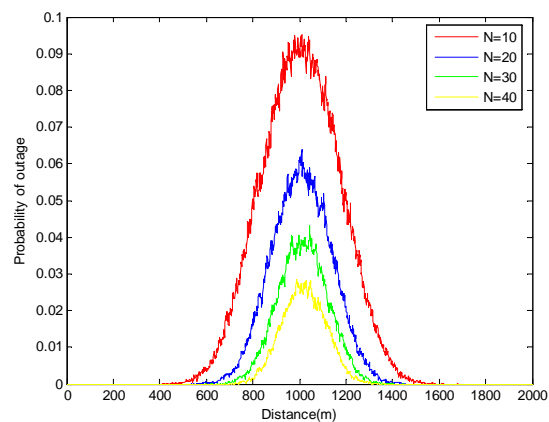
Fig. 2a Effect of window size on Probability of outage for given \rho = 0.5, \sigma = 8 dB, \eta = 3.6
