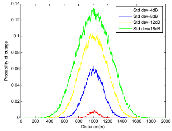
Fig. 4a Effect of standard deviation on probability of outage for given \eta = 3.6, \rho = 0.5, N = 20
