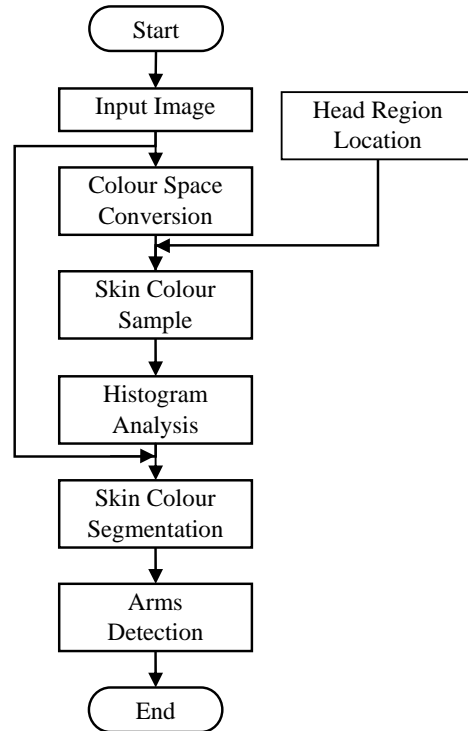
Fig. 1 Flowchart of the histogram-based skin colour segmentation
