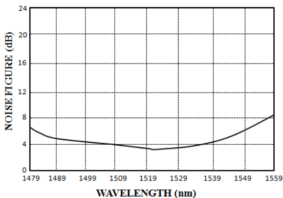
Fig. 7 Noise Figure versus Wavelength of HTE
