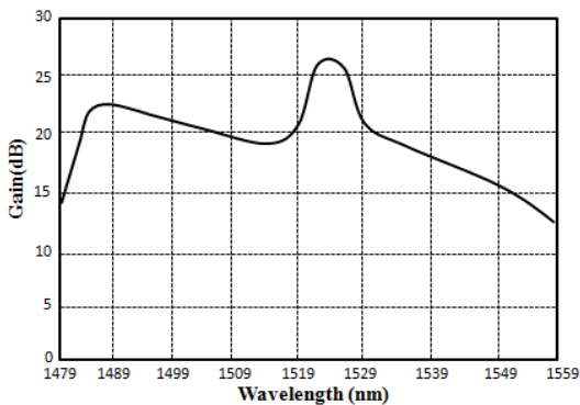
Fig. 6 Gain versus Wavelength of HTE
