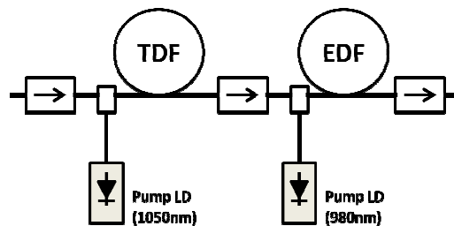
Fig. 5 Schematic arrangement of HTE
