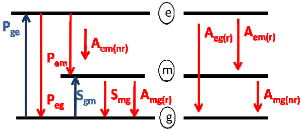
Fig. 1 Three level energy diagram of EDFA
