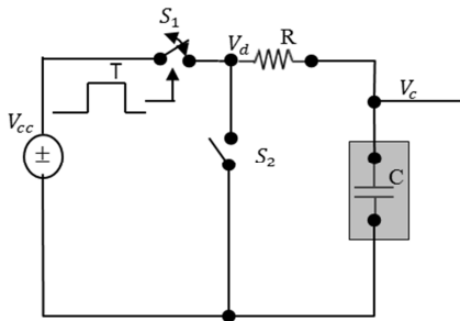
Fig. 5 Charging stage circuit
