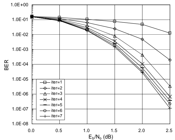
Fig. 6 BER of Type II
