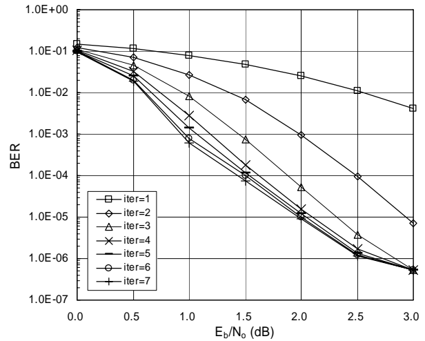
Fig. 5 BER of Type I
