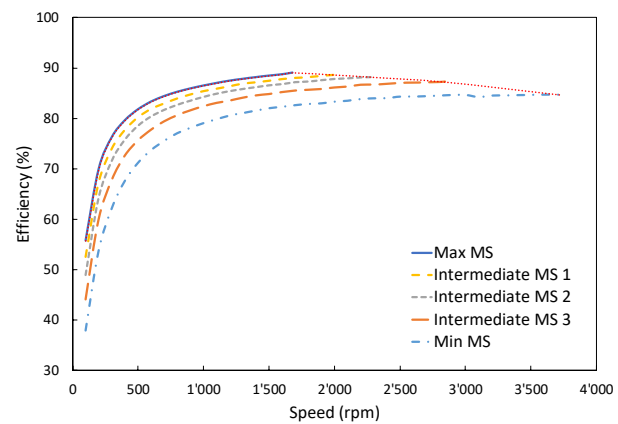
Fig. 12 Measured motor efficiency for different magnetization states
