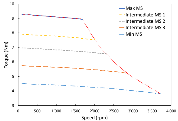
Fig. 11 Measured torque-speed characteristics under nominal current for different magnetization states ( i_d=0 , i_q=I , V_{DC} = 600 V )
