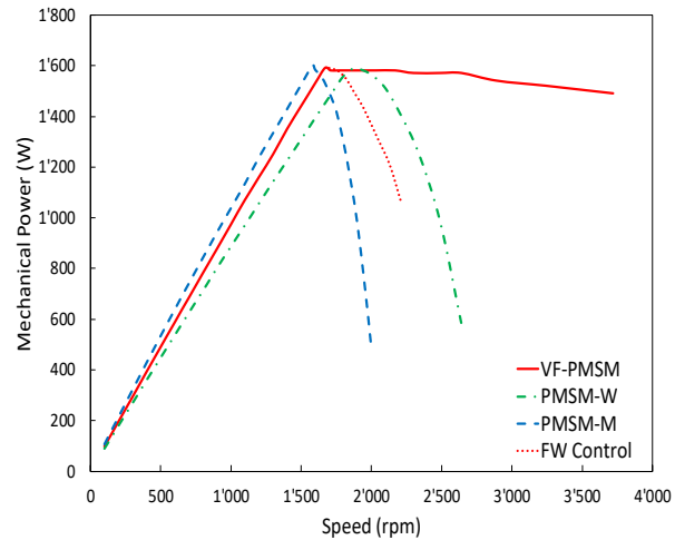
Fig. 14 Measured mechanical power of PMSM
