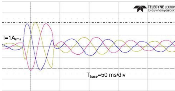
Fig. 10 Transient stator currents in demagnetization process
