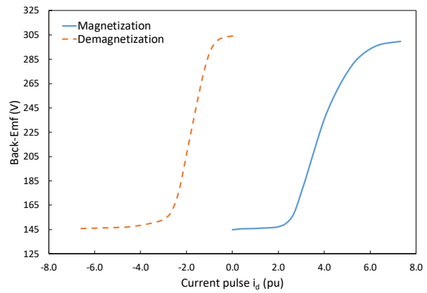
Fig. 8 Measured magnetization and demagnetization characteristic of VF-PMSM at 1500 rpm
