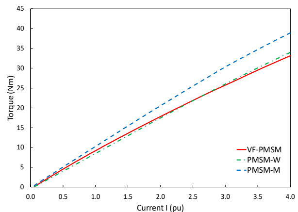
Fig. 15 Comparison of measured characteristics torque-current at 100 rpm
