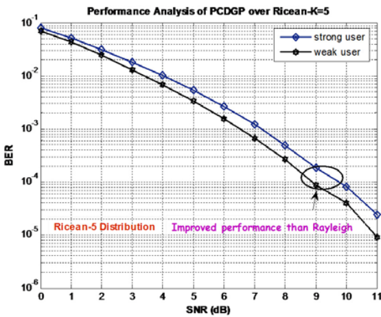
Fig. 5. Simulation results for the PCDGP system for both users over Ricean-5 fading channel
