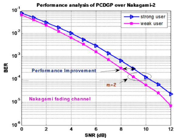
Fig. 3. Simulation results for the PCDGP system for both users over Nakagami-2 fading channel
