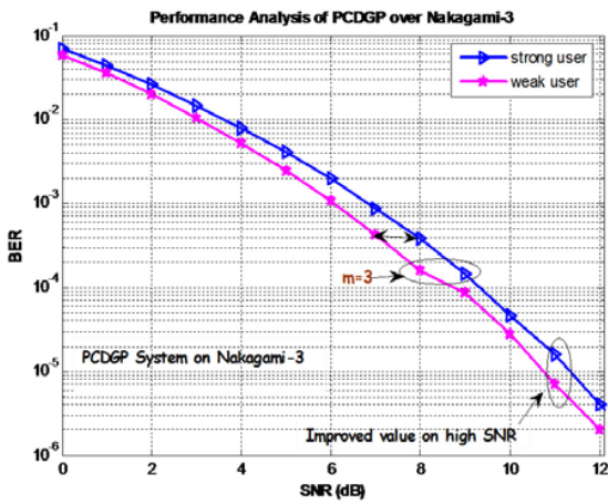
Fig. 4. Improved simulation results for the PCDGP system for both users over Nakagami-3 fading channel
