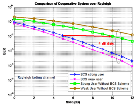
Fig. 7. The comparison of two-hop cooperative system between with and without BCS scheme
