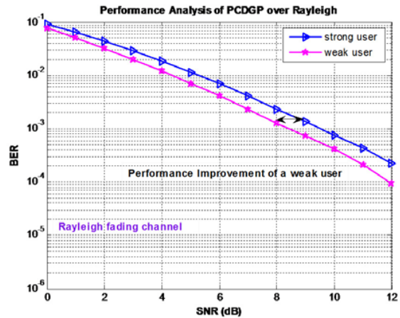
Fig. 2. Simulation results for the PCDGP system for both users over Rayleigh fading channel
