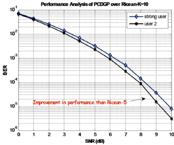
Fig. 6. Improved simulation results for the PCDGP system for both users over Ricean-10 fading channel
