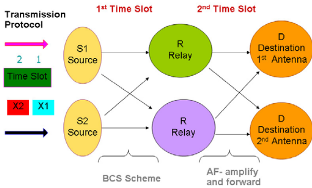
Fig. 1. Illustration of MIMO wireless network in Power and Cooperation Diversity gain mode with two source terminals S , two relays and the destination terminal D with two antennas
