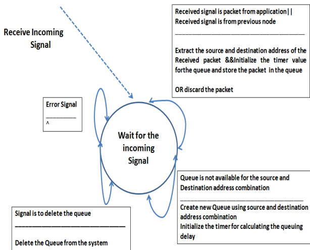
Fig. 3 FSM for Queue Control Mechanism
