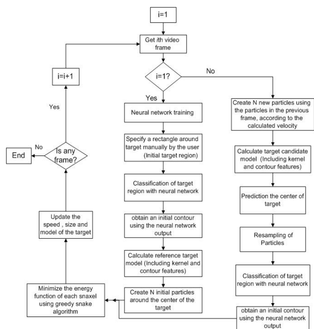
Fig. 1 The flowchart of proposed algorithm. Our proposed method is made in three steps: (1) estimate the target location by particle filter, (2) segmentation target region using neural network, and (3) find the exact contours by greedy snake algorithm
