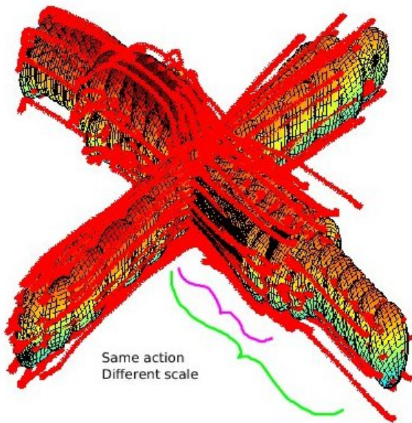
Fig. 2: Data covered with Gaussians.
