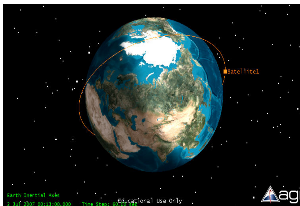
Fig. 1 ICUBE-1 Orbit in STK
