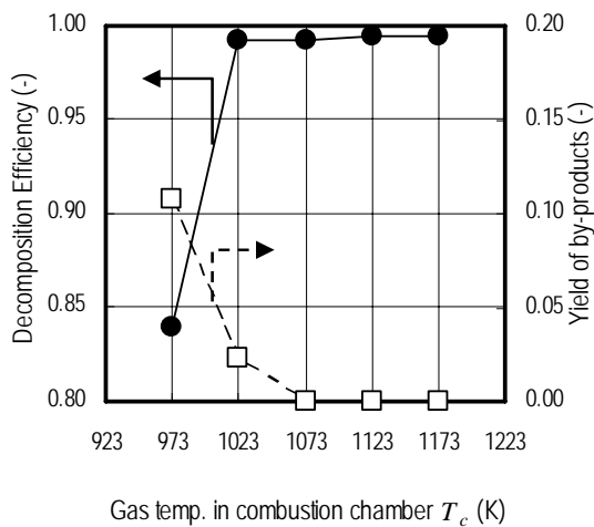
Fig. 3 Effect of gas temperature on toluene decomposition efficiency
