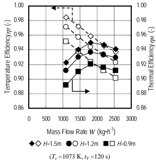
( T_c = 1073 \text{ K} , t_v = 120 \text{ s} ) Fig. 4 Effect of the mass flow rate W on \eta_T and \eta_H
