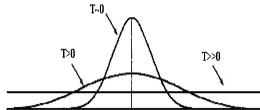
Fig. 1 Distribution of probability for three different temperatures
