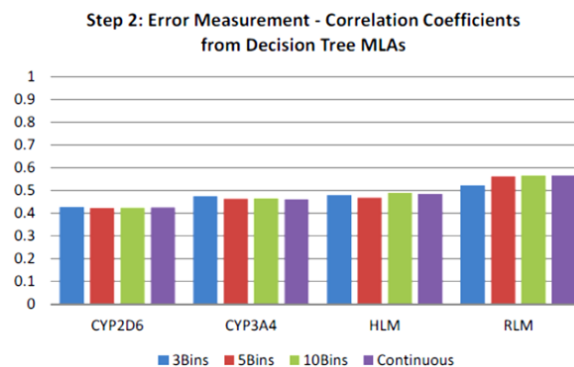
Fig. 10 Discretization CC DT
