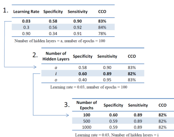
Fig. 17 HLM NN Optimization
