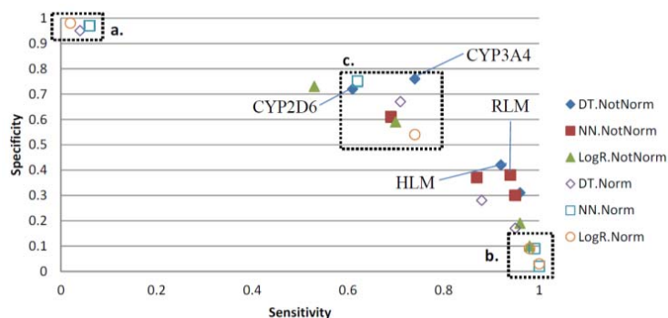
Fig. 14 Normalization Sensitivity vs. Specificity
