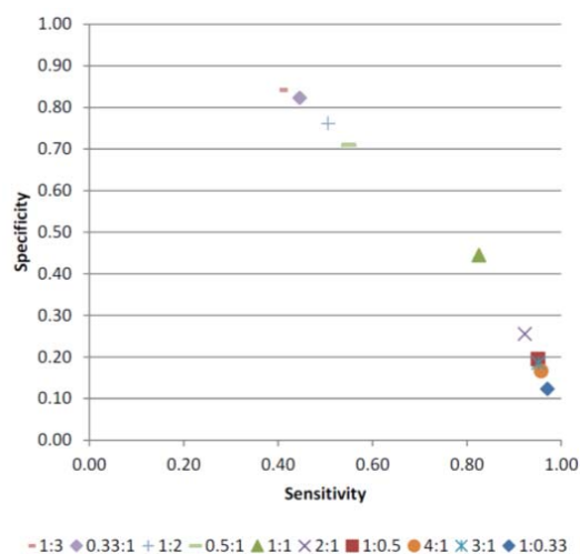
Fig. 15 Over-/Under-sampling Sensitivity vs. Specificity
