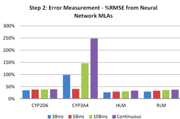
Fig. 9 Discretization %RSMC NN
