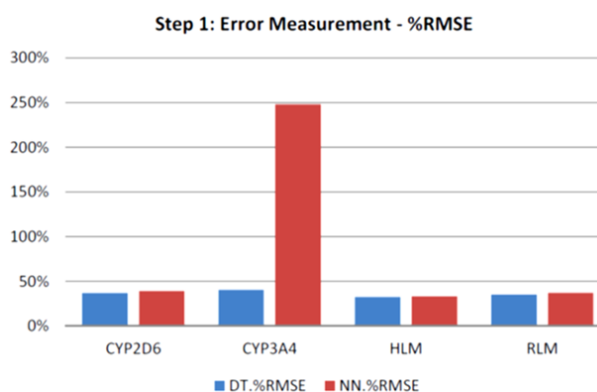
Fig. 6 Instance Selection %RMSE
