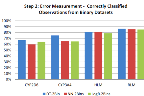
Fig. 12 Discretization CC Binary Bin
