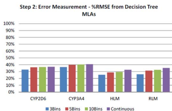
Fig. 8 Discretization %RSMC DT
