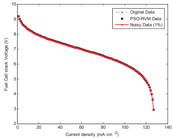
Fig. 6 Voltage-current curves
