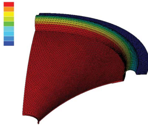
Fig. 8 Mode of vibration displacement for Optimal Solution A at 1500 Hz
