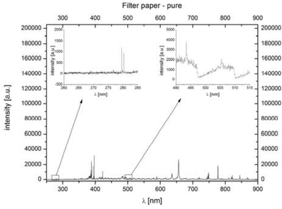
Fig. 2 LIBS spectrum of pure Filter paper
