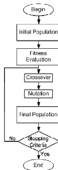
Fig. 1 Flowchart of optimizing electrospinning parameters using genetic algorithm
