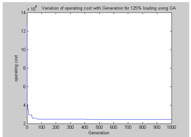
Fig. 3 Variation of Total Cost with Generation for 125% Reactive loading
