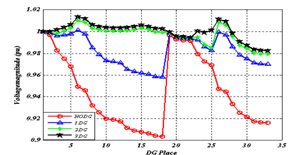
Fig. 7. Voltage profile of 33-bus test system in presence of type 2 DG unit(s)
