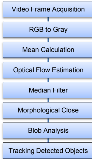
Fig. 1 Block diagram of the proposed algorithm
